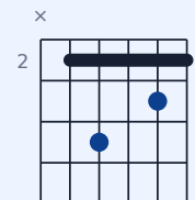
Sim7 (Bm7)
