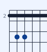
FA#m (F#m)
